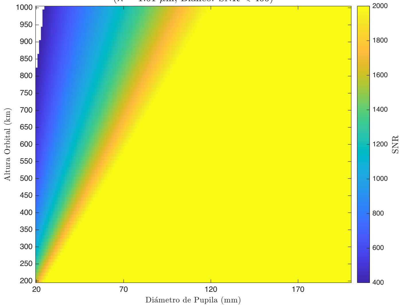
SNR - Cassegrain - Detector 3 ( \lambda = 1.61 \mu\text{m} , Blanco: \text{SNR} < 400 )
